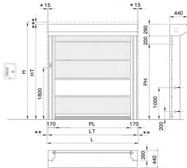
Dimensional specifications
